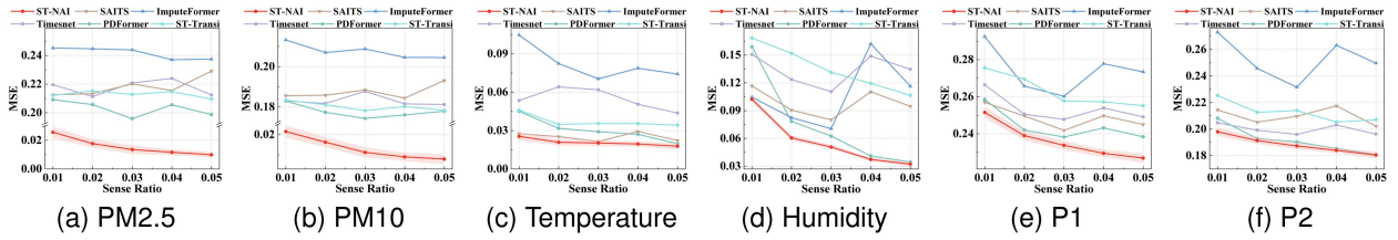
Fig. 9. Inference performance under different sense ratios with multi-scale inputs. (a) PM2.5. (b) PM10. (c) Temperature. (d) Humidity. (e) P1. (f) P2.
