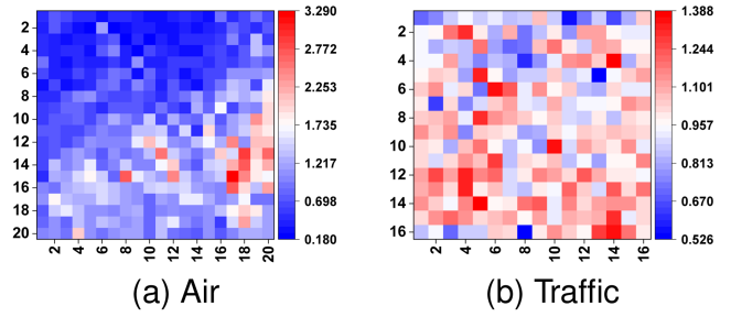
Fig. 16. Visualization of spatial importance. (a) Air. (b) Traffic.
