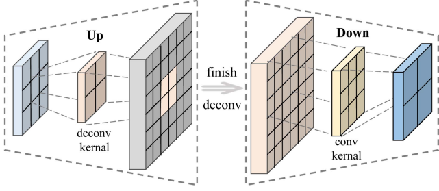
Fig. 5. The example of the Scale-Adjusted Resampling.
