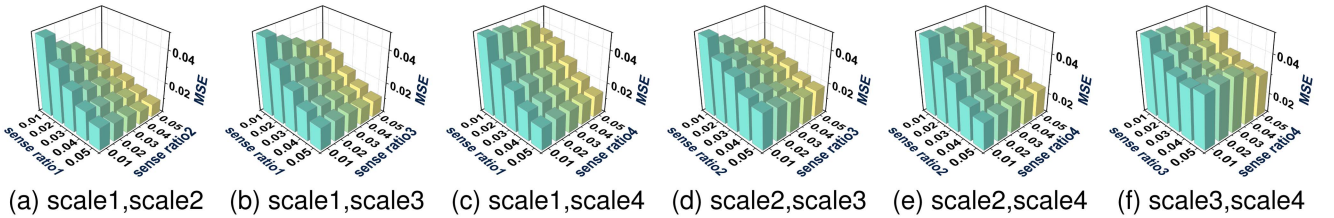
Fig. 10. Inference performance under two different scales. (a) scale1,scale2. (b) scale1,scale3. (c) scale1,scale4. (d) scale2,scale3. (e) scale2,scale4. (f) scale3,scale4.
