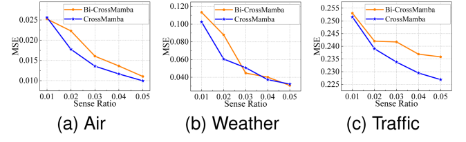
Fig. 13. Comparison between CrossMamba and Bi-CrossMamba. (a) Air. (b) Weather. (c) Traffic.
