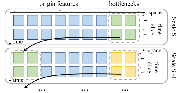
Fig. 8. The example of the Cross-Mamba.
