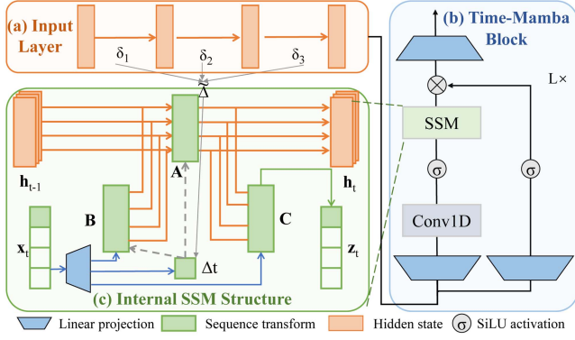
Fig. 4. The structure of the Time-Mamba. Irregular observations are first processed by (a) the Input Layer, then propagated to (b) the Time-Mamba Block for temporal modeling, whose internal mechanism is illustrated in (c) as the Internal SSM Structure.
