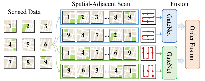
Fig. 7. The structure of the Spatial-Adjacent Scan.
