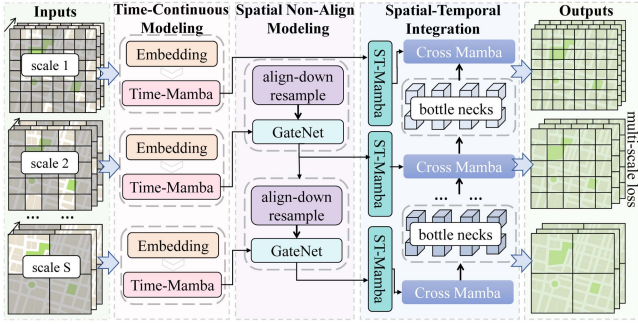
Fig. 3. The structure of the ST-NAI.
