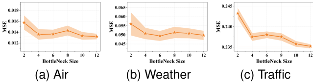
Fig. 15. Parameter Sensitivity Analysis of Bottleneck Size. (a) Air. (b) Weather. (c) Traffic.
