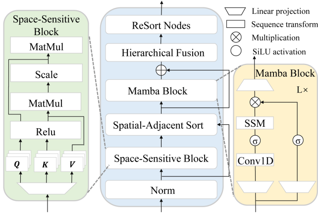
Fig. 6. The structure of the ST-Mamba.
