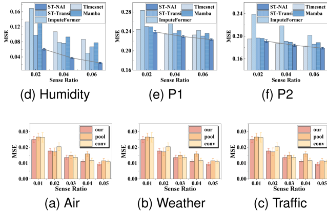
Fig. 12. Performance of Scale-Adjusted Resampling. (a) Air. (b) Weather. (c) Traffic.
