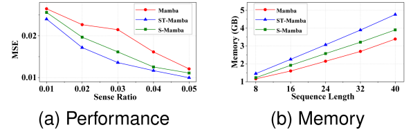
Fig. 14. Ablation of the ST-Mamba. (a) Performance. (b) Memory.
