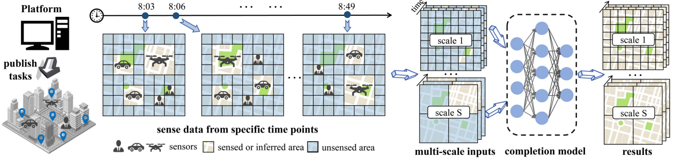
Fig. 2. The workflow of our work: the platform recruits users to collect partial multi-scale data at specific timestamps for data inference.
